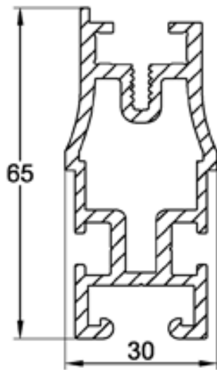
14 065 rackarm 65
