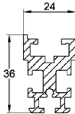
14 036 rackarm 36
