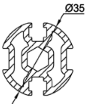
14 035 drive tube 35
